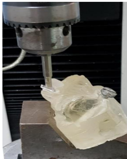
Figure 6 Fracture resistance test
